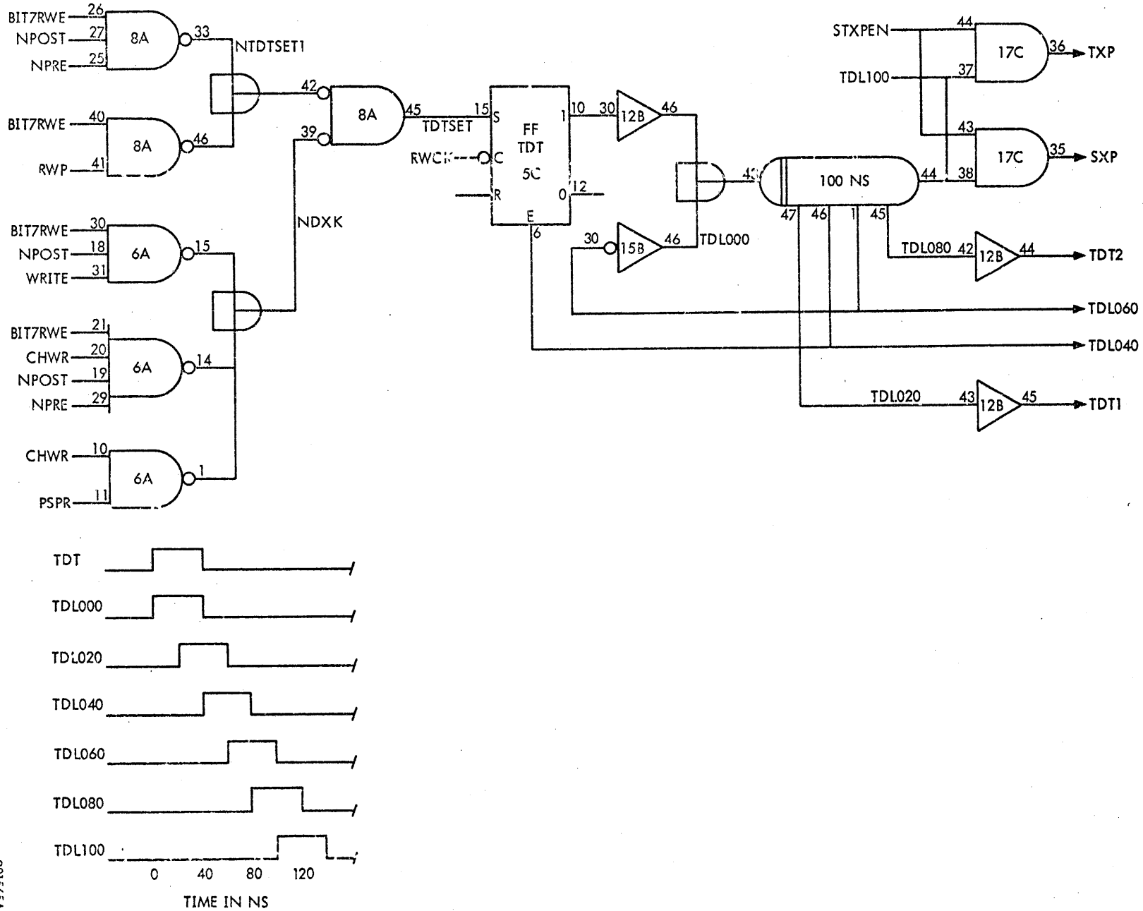
Figure 4-16. TDL Delay Line, Logic and Timing Diagram
