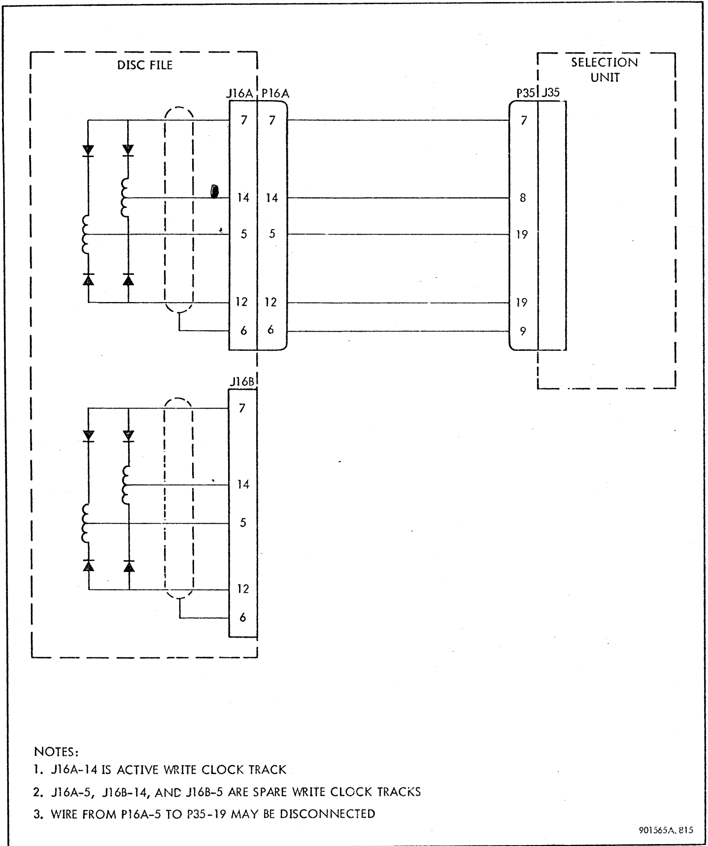
Figure 8-14. Write Clock Tracks, Schematic Diagram
