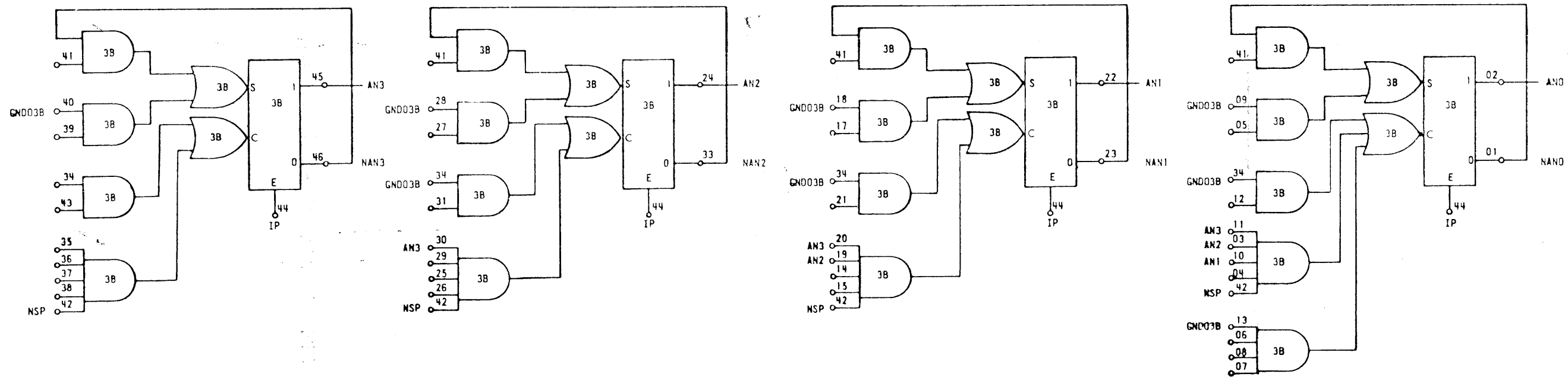
Figure 6-9. IP RAD Selection Unit, Angle Register, Logic Diagram 901565A, 610
