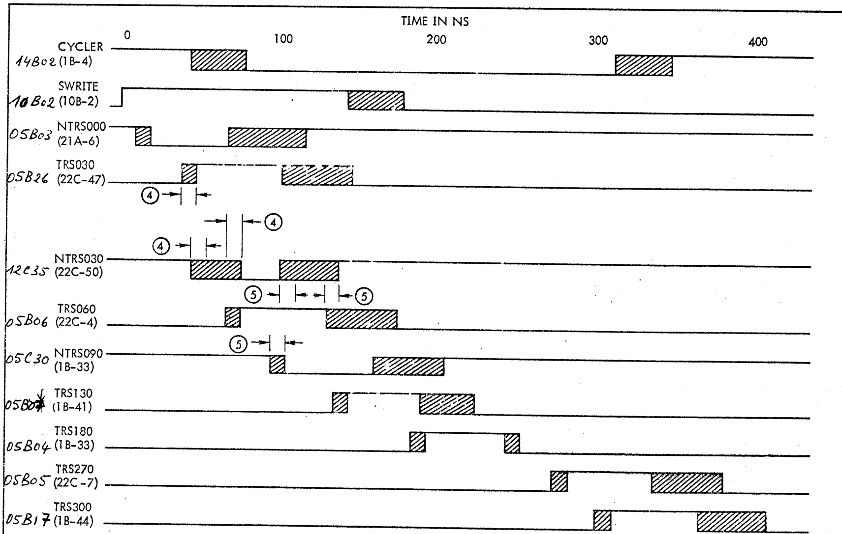
Figure 8-11. TRL Delay Line Signals, Timing Diagram
