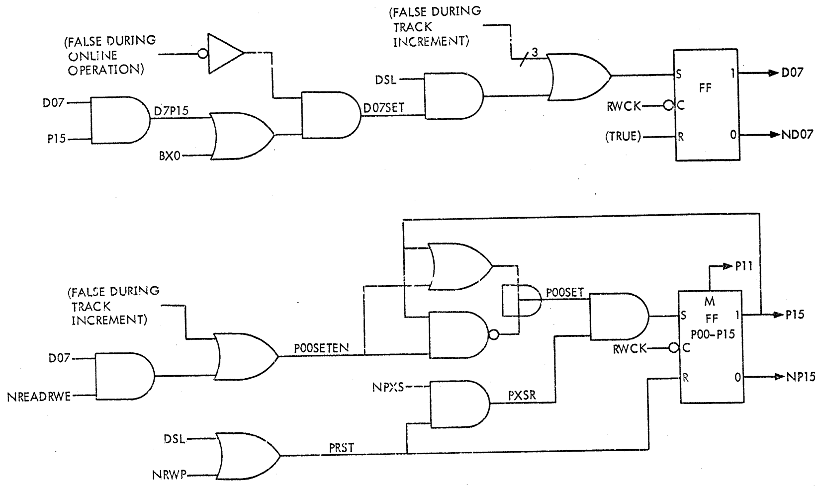
Figure 4-19. Address Incrementation, Simplified Logic Diagram
