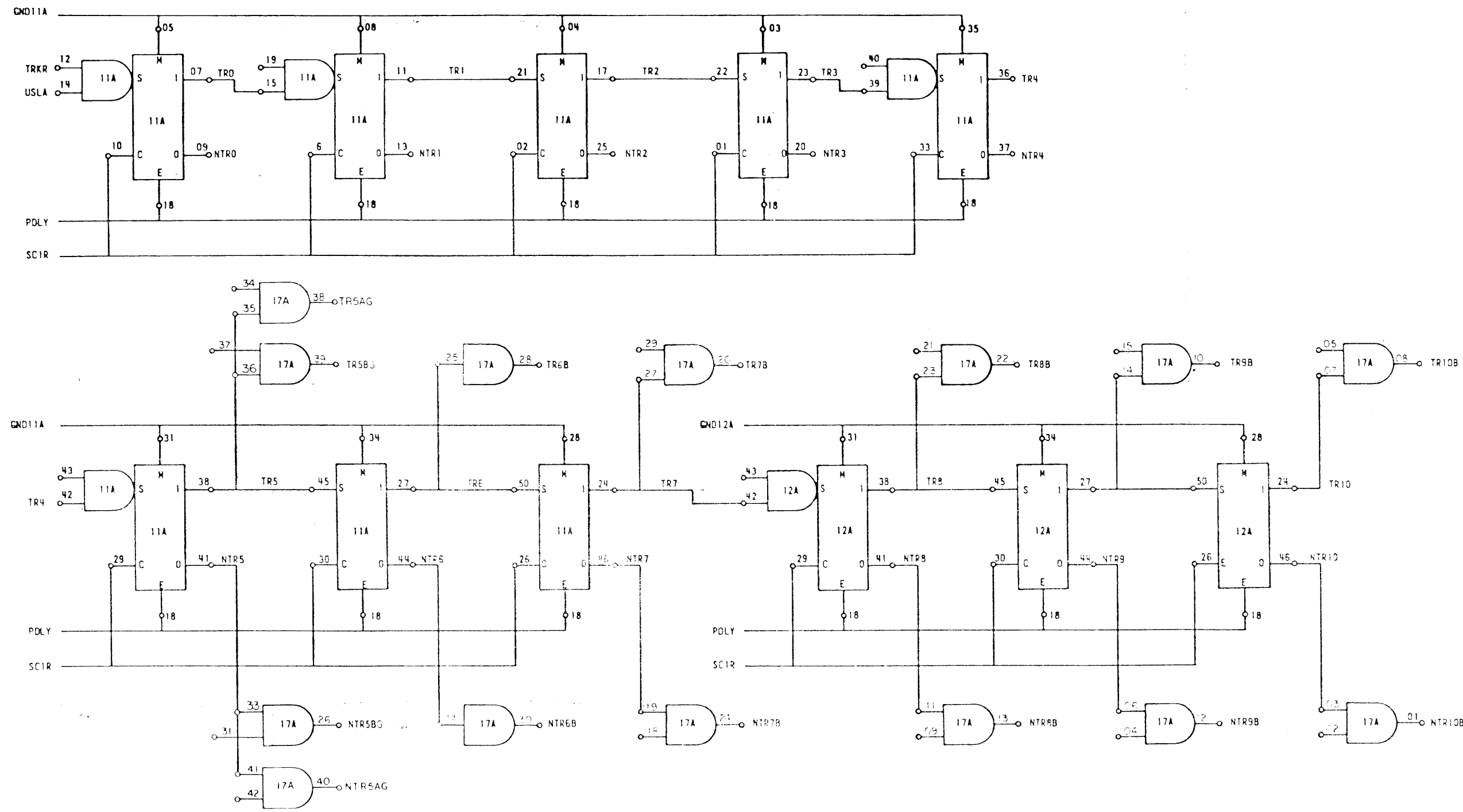
Figure 6-18. EP RAD Selection Unit, Track Register (With Logical Sparring), Schematic Diagram 901565A.618
