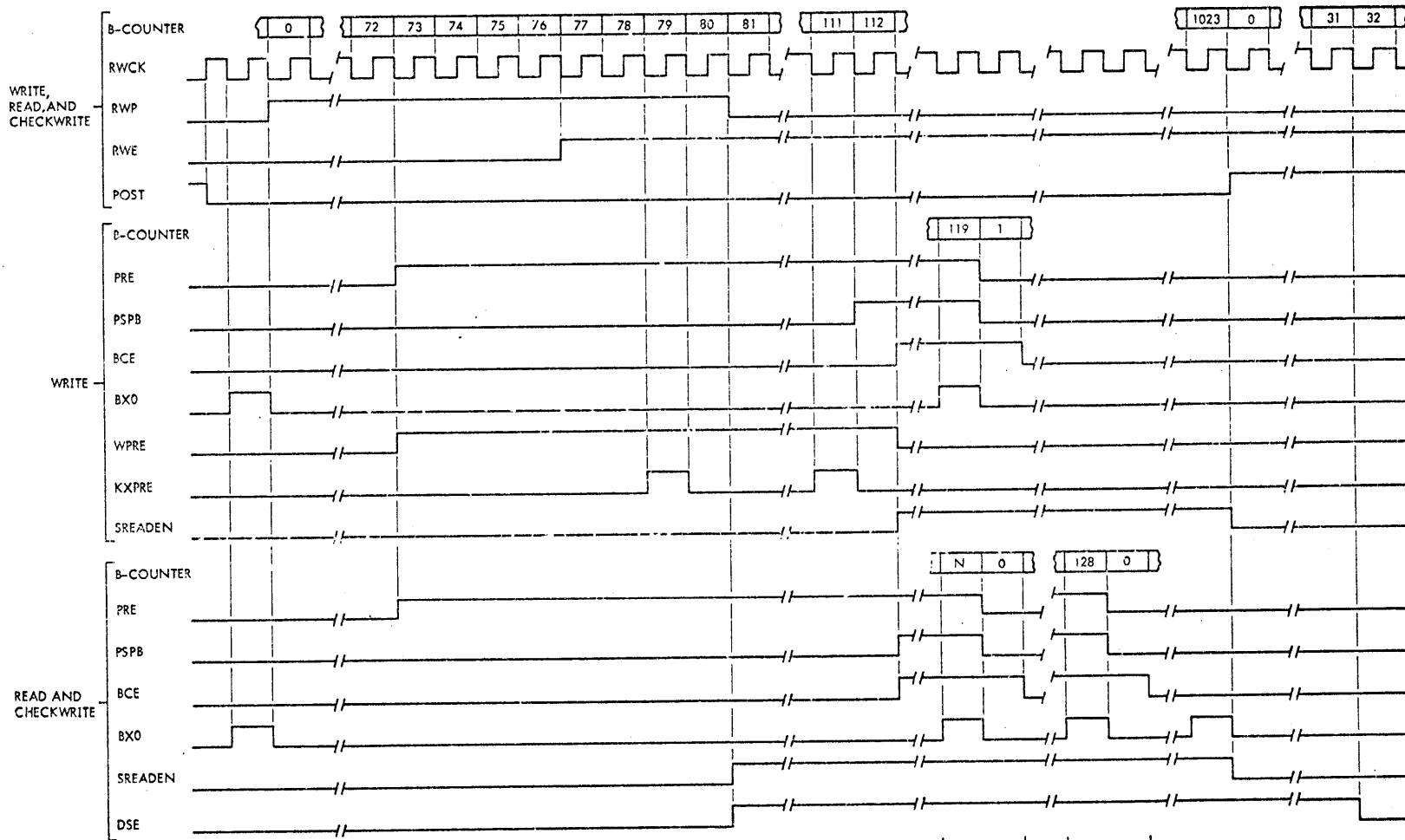
Figure 4-18. Interface Control Circuits, Timing Diagram
