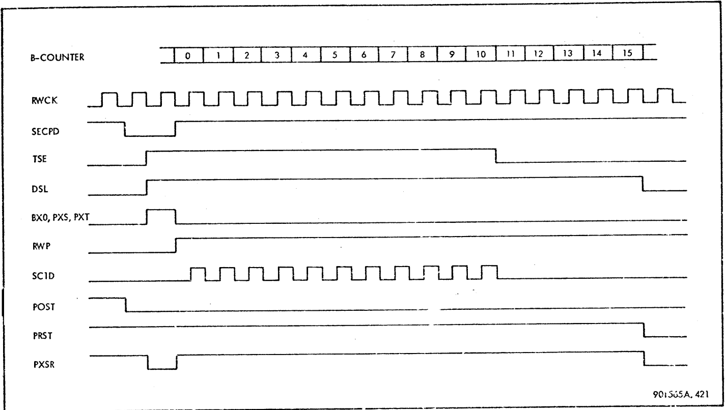
Figure 4-17. Track Shift Sequence, Timing Diagram
