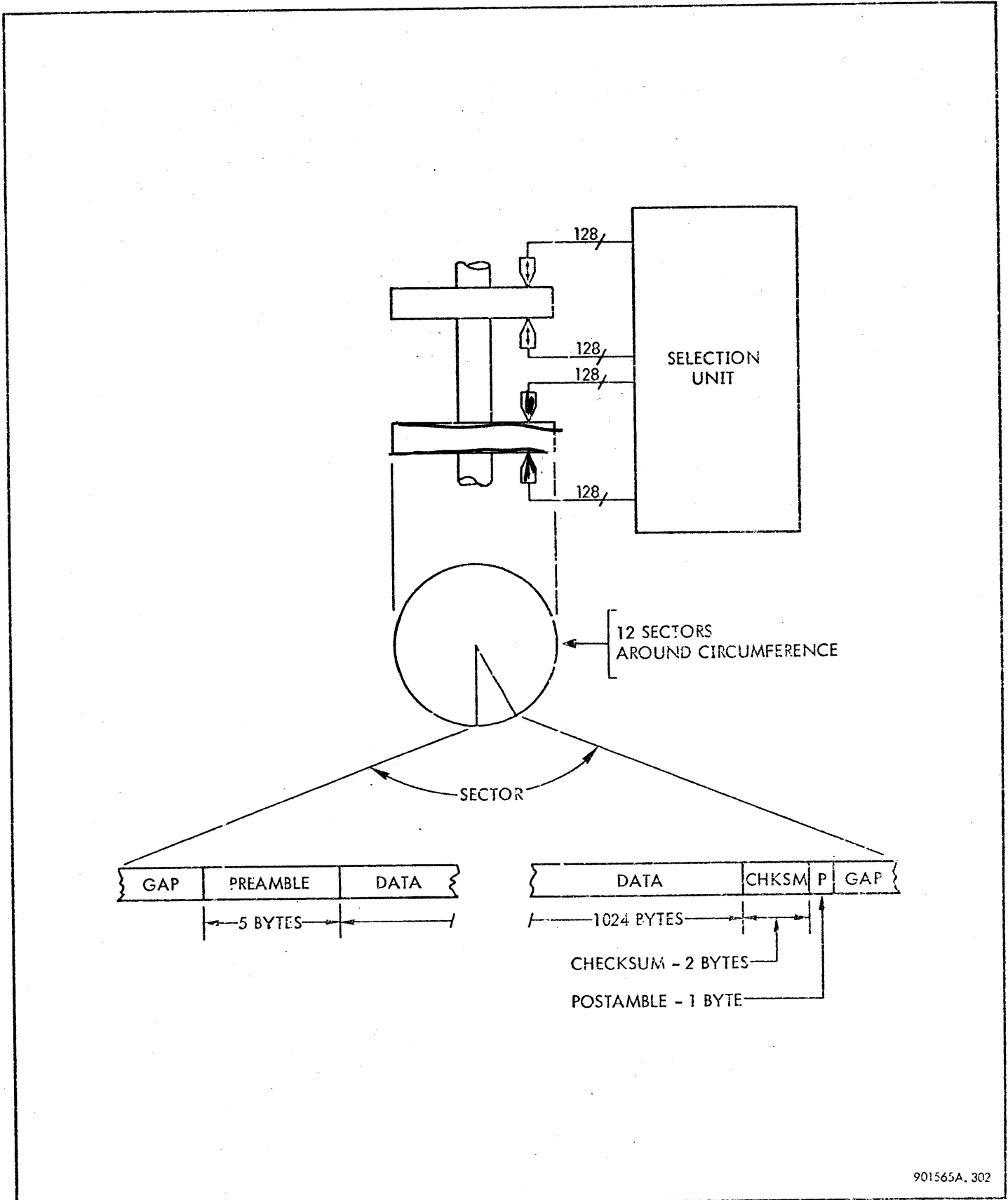
Figure 3-2. EP RAD Disc File, Data Organization
