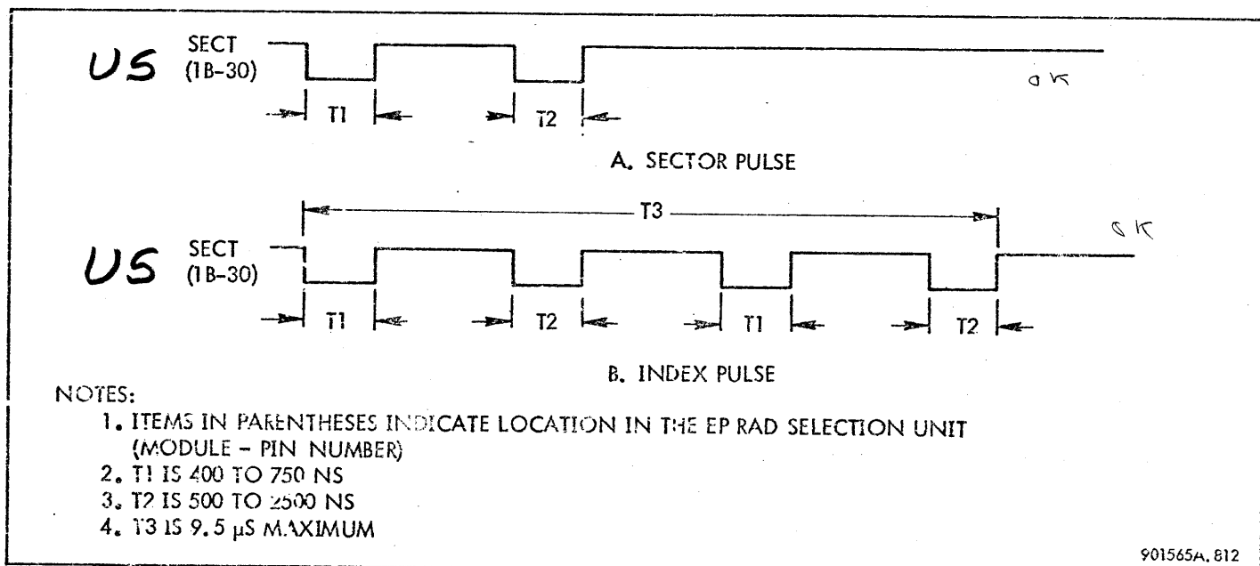
Figure 8-2. Signal SECT, Timing Diagram
