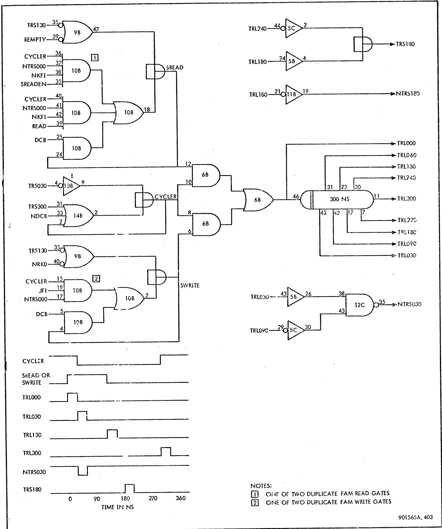
Figure 4-13. TRL Delay Line, Logic and Timing Diagram
