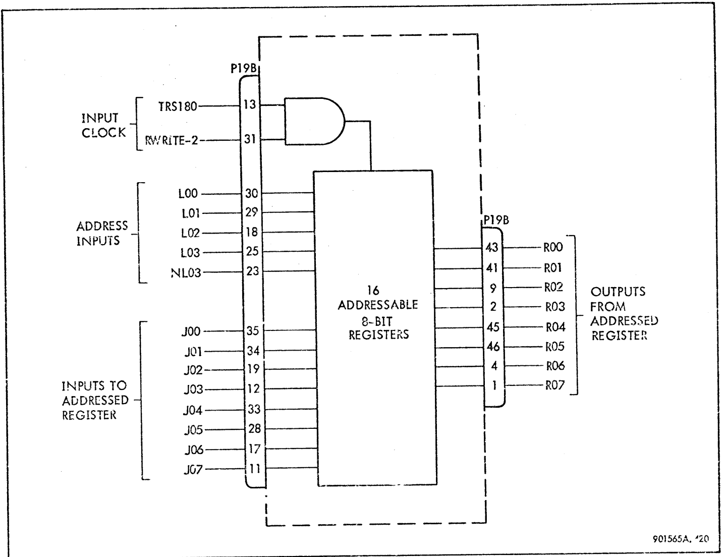
Figure 4-12. FAM Module, Block Diagram
