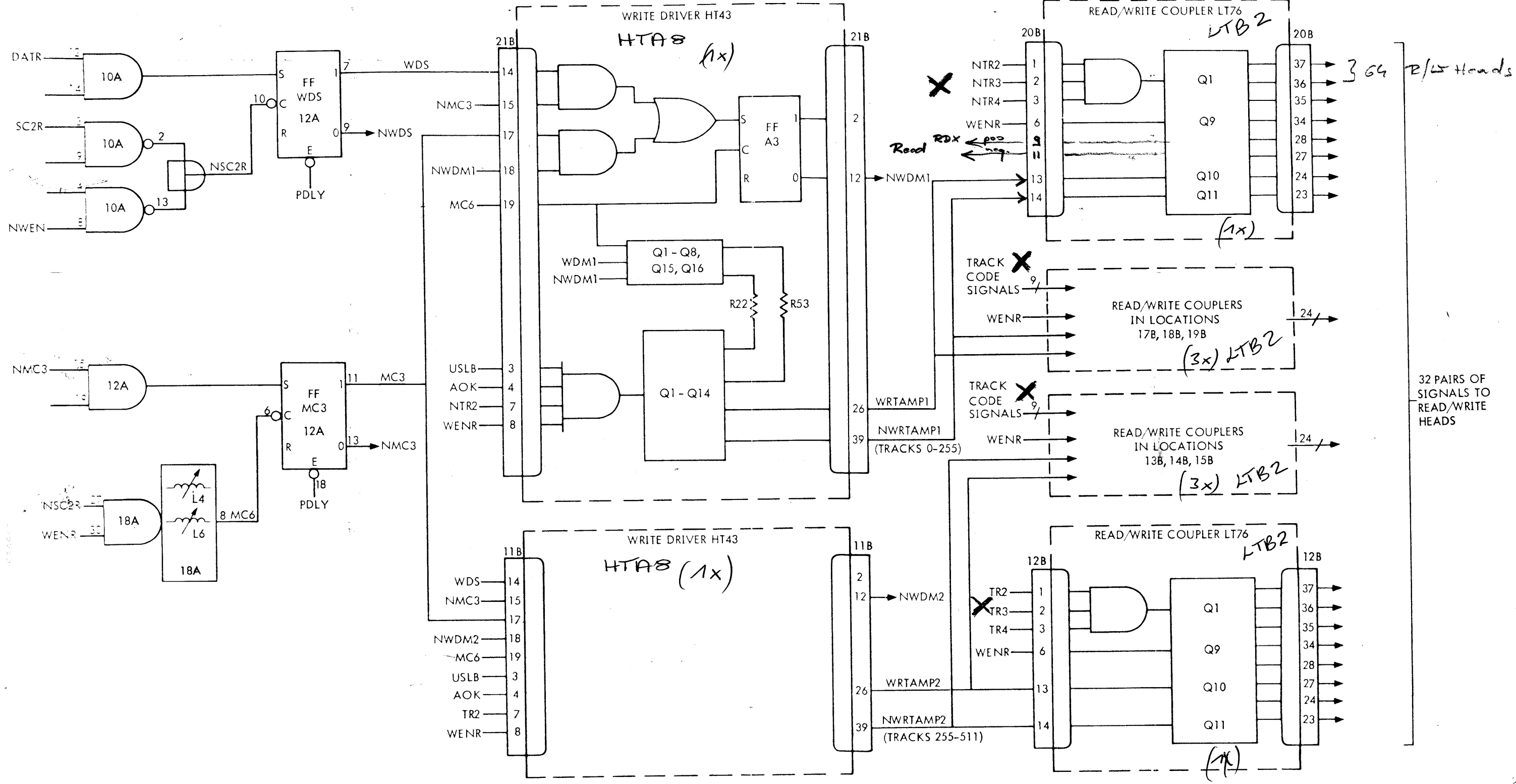
Figure 4-28. Write Channel, Schematic Diagram
