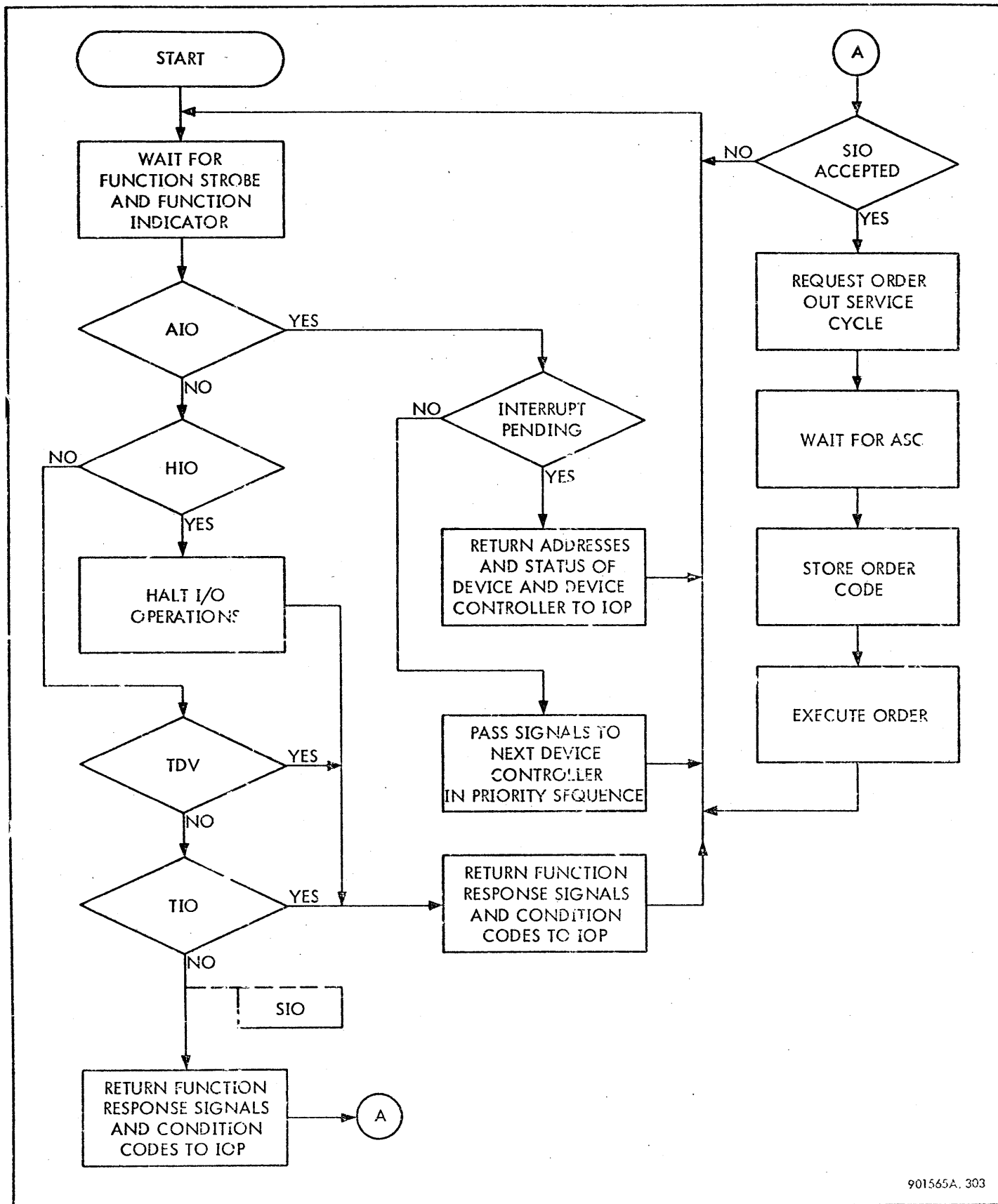
Figure 3-3. Response to IOP Commands, Flow Diagram
