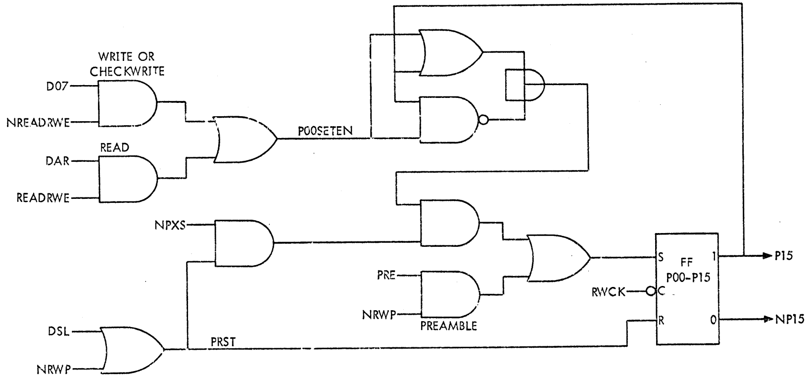
Figure 4-20. Checksum Generation, Simplified Logic Diagram
