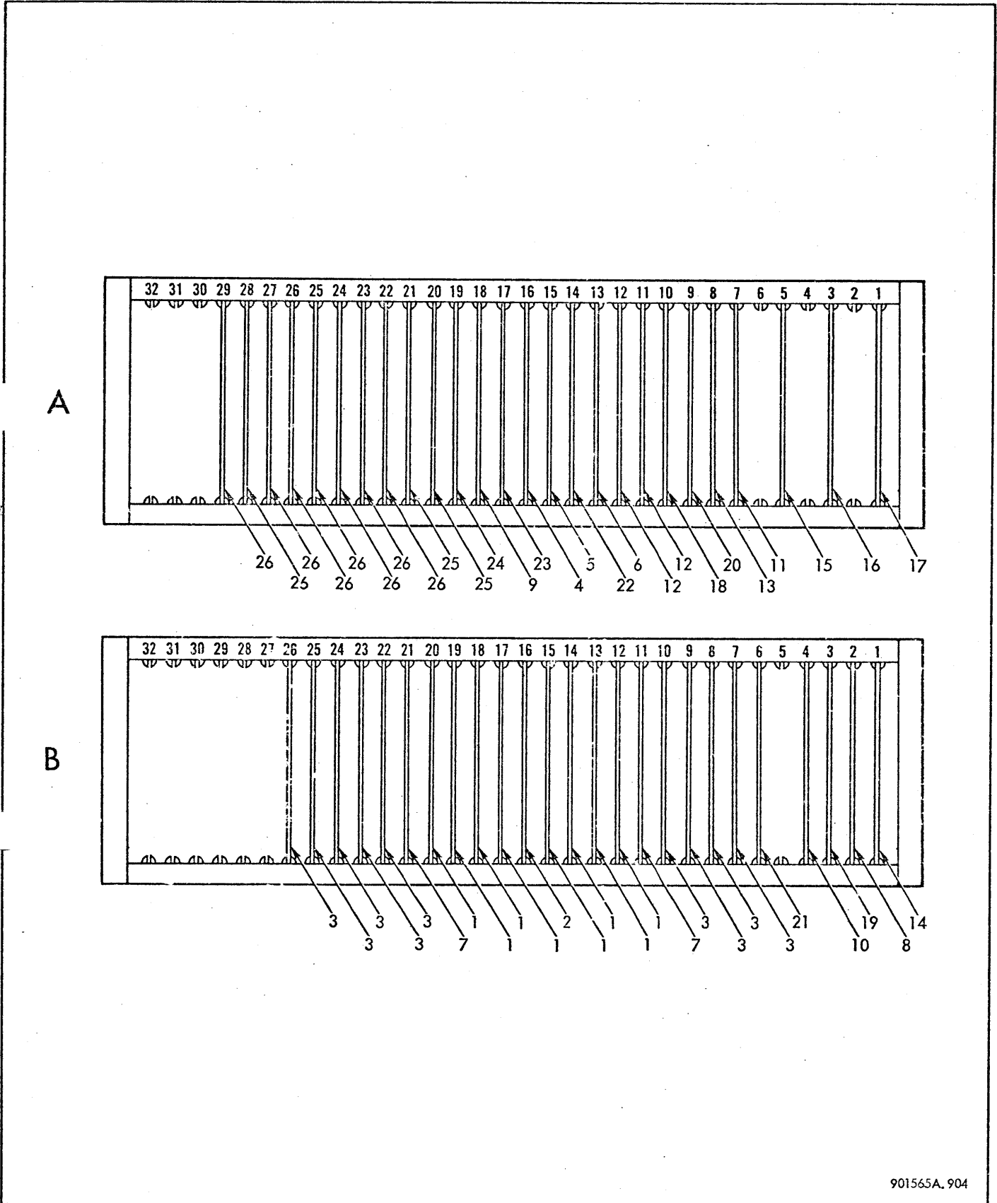
Figure 9-4. Module Location (Selection Unit Assembly)
