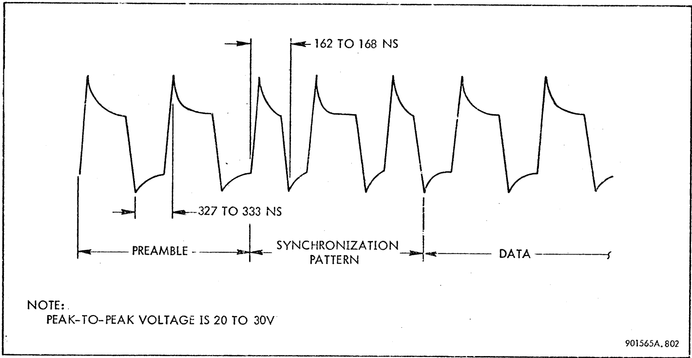
Figure 8-12. Write Amplifier Output Signals, Timing Diagram
